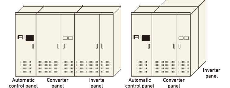
Side by side arrangement [ 6MVA model ]
