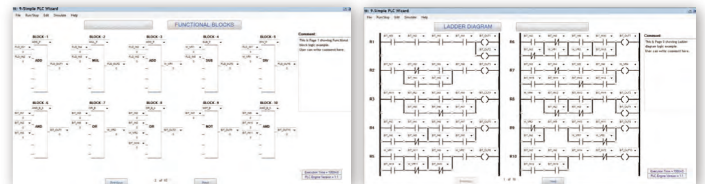
User-defined functions
