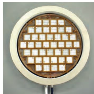
9MVA model IEGT power device
